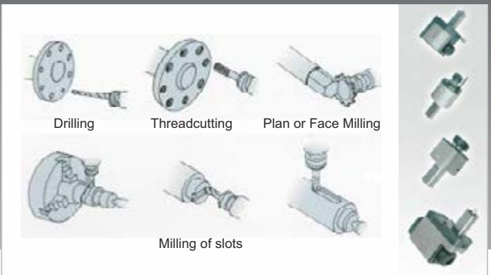
Radial Driven Tool BMT tooling system
